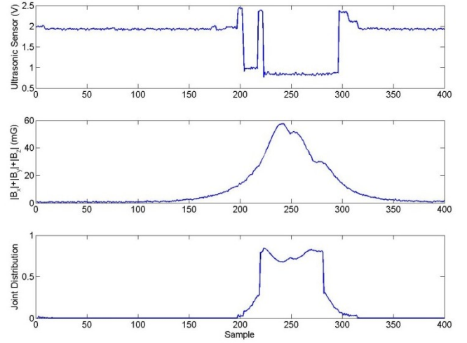
Fig 19. Joint likelihood of vehicle presence
