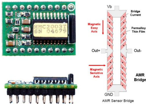
Fig 2. HMC 2003 Magneto-resistive sensor
