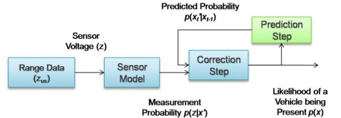
Fig 15. Bayesian filter algorithm (individual sensor)
