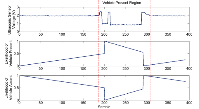
Fig 14. Ultrasonic sensor predictive model
