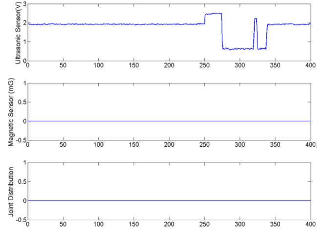
Figure 20. Joint likelihood of a non-metallic object
