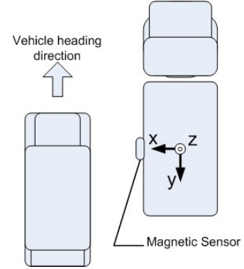
Fig 3. Road test configuration
