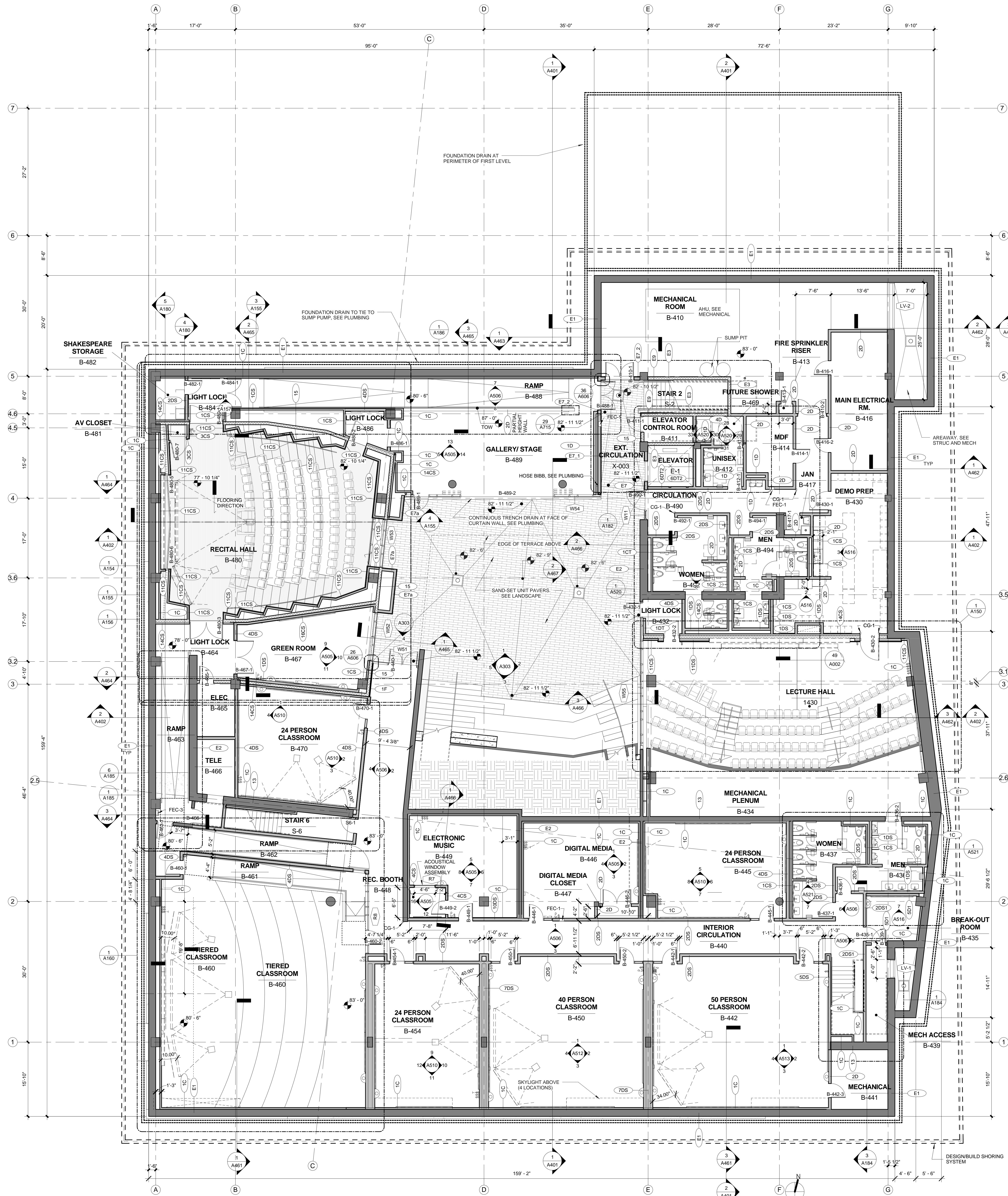
1 LEVEL 0 FLOOR PLAN 1/8" = 1'-0"
